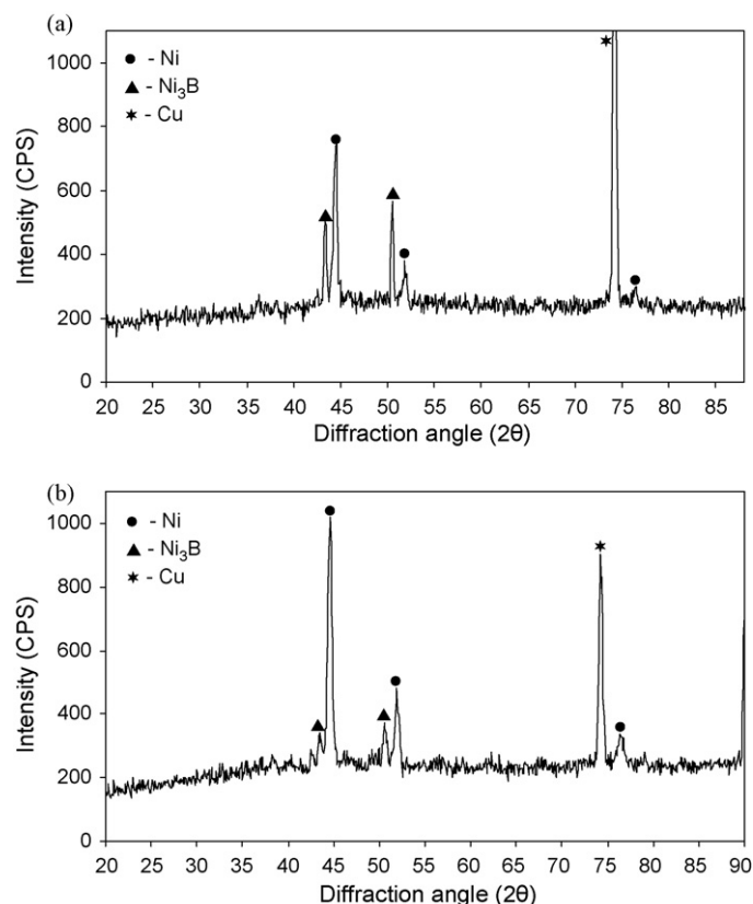
Fig. 3. X-ray diffraction patterns of ED Ni-B and Ni-B-Si 3 N 4 composite coatings after heat-treatment at 400 °C for 1 h: (a) ED Ni-B; and (b) ED Ni-B-Si 3 N 4 .
